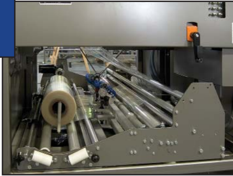
Low height slide out film rack for easy film loading
